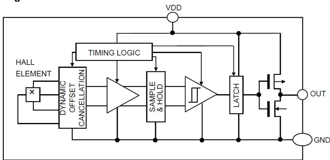
Figure 3, Block Diagram of AS1515
