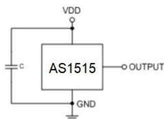
Figure 1, Typical Application Circuit of AS1515
