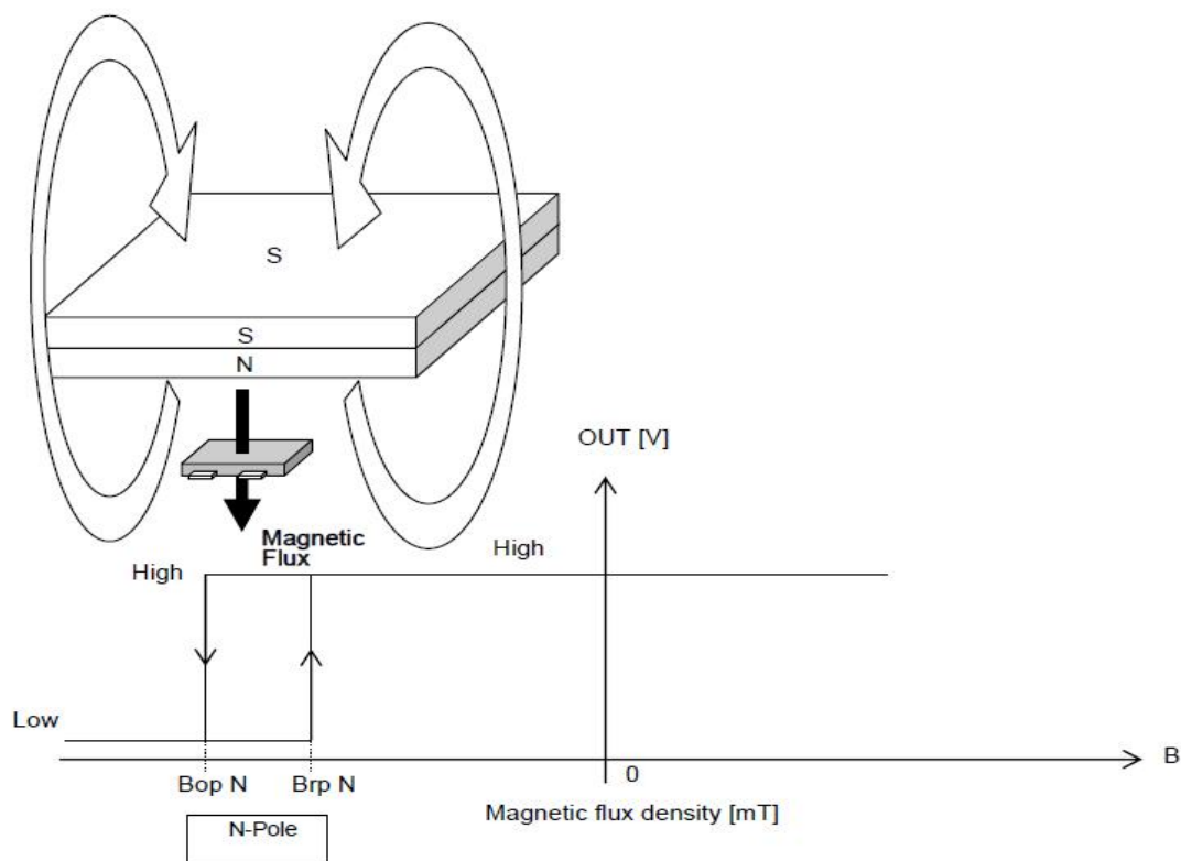
Fig 4, Magnetic Operation Characteristic of AS1515
